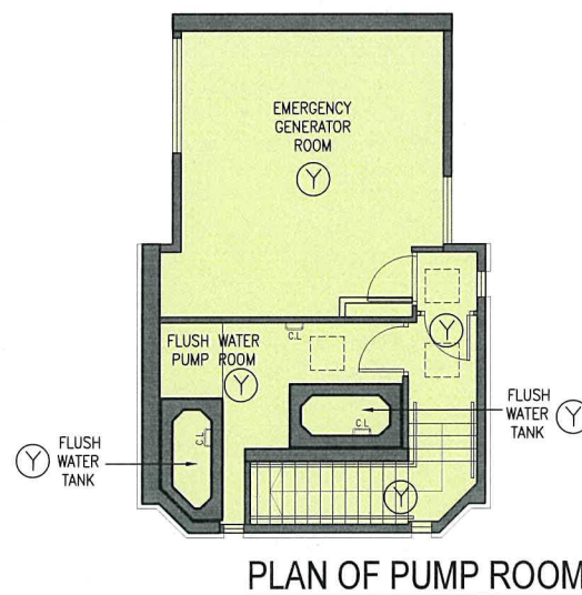
PLAN OF MACHINE ROOM
